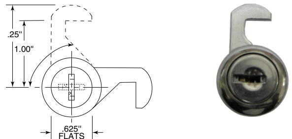
38077-15 (Towel Dispenser)
