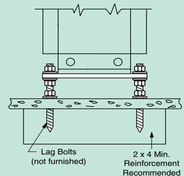
PLYWOOD FLOOR
