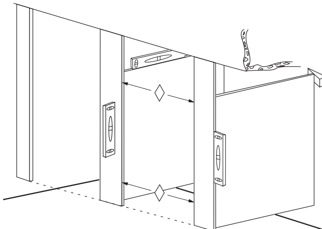
Fig. 6c: Ceiling-Hung Installation.
