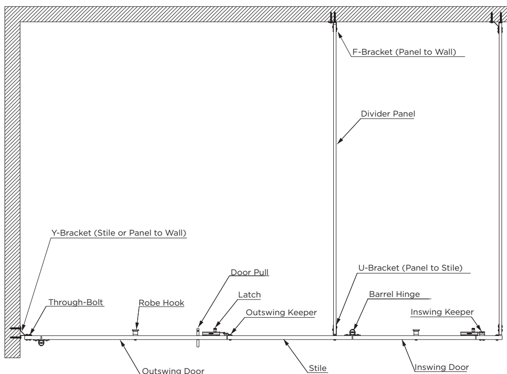
Top View of 1092 (Barrel Hinge and Standard Bracket) installation.
