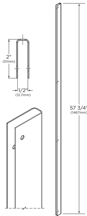
#1001368 U-Channel
