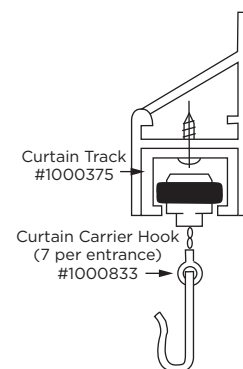
Fig. 7b: Curtain Track
