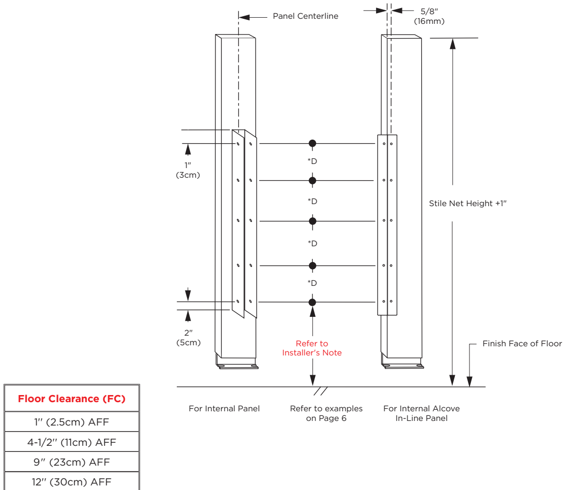
Fig. 5a: Overhead-Braced Stiles.
