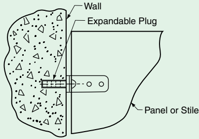
Masonry Wall
